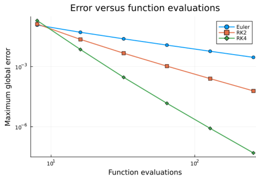
Figure 8: Maximum global error as a function of total function evaluations, demonstrating the improved efficiency of higher-order methods.
