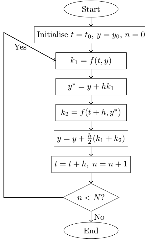
Figure 2: General flowchart for the RK2 algorithm.
